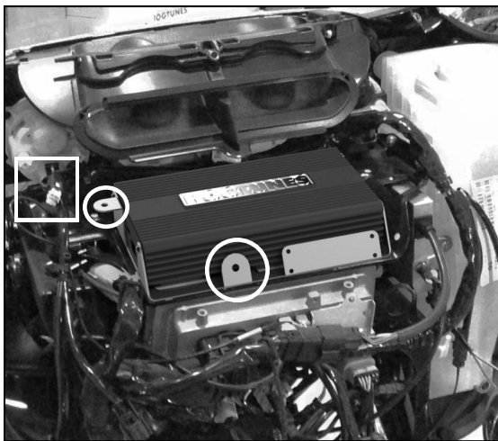
Fig 1.2: Amplifier and mounting plate correctly oriented. The plate with 4 small holes is for mounting a popular factory accessory. The white circle show tabs which are there for the factory “Christmas Tree” fasteners to re-secure the harnesses lifted earlier.
